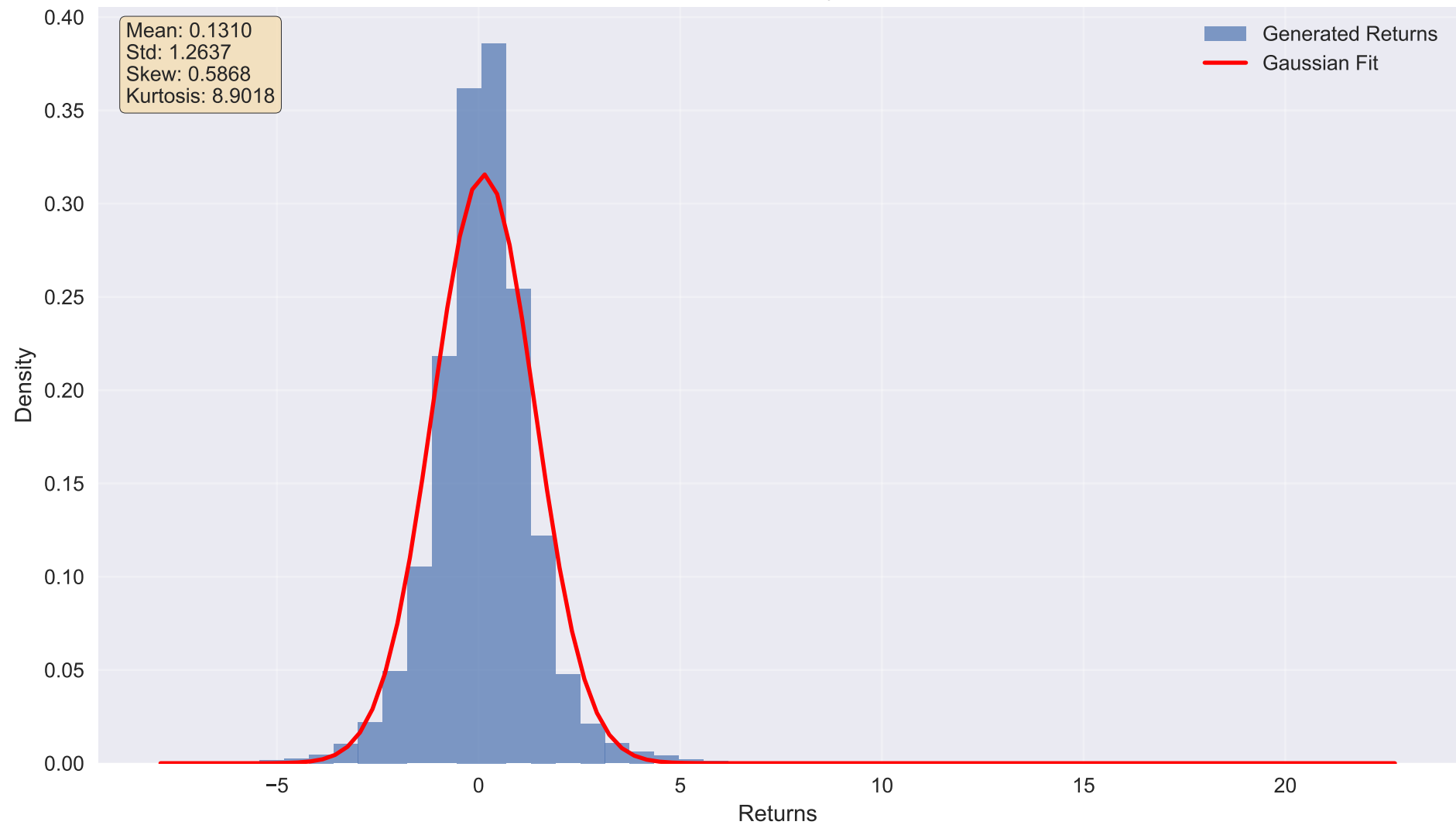
Zero Conditioned: Stylized Facts
